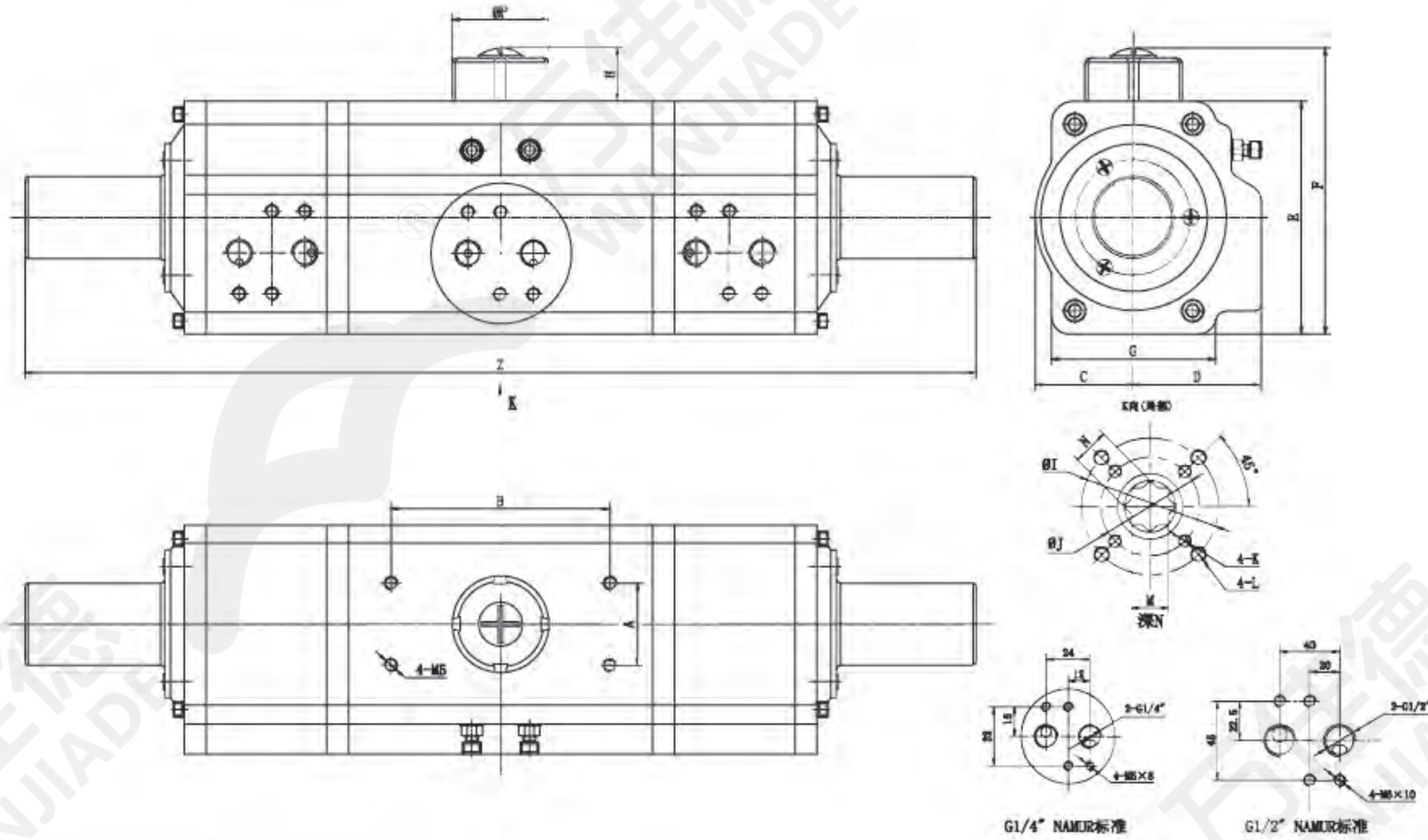
外形及连接尺寸 Shape and connection size
